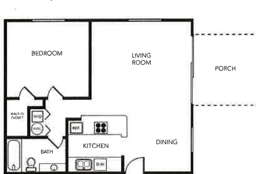
CLAM - UNIT F 1 BEDROOM | 1 BATH 701 SQ.FT. Units: 110, 210, 114, 214, 116, 216, 120, 220
